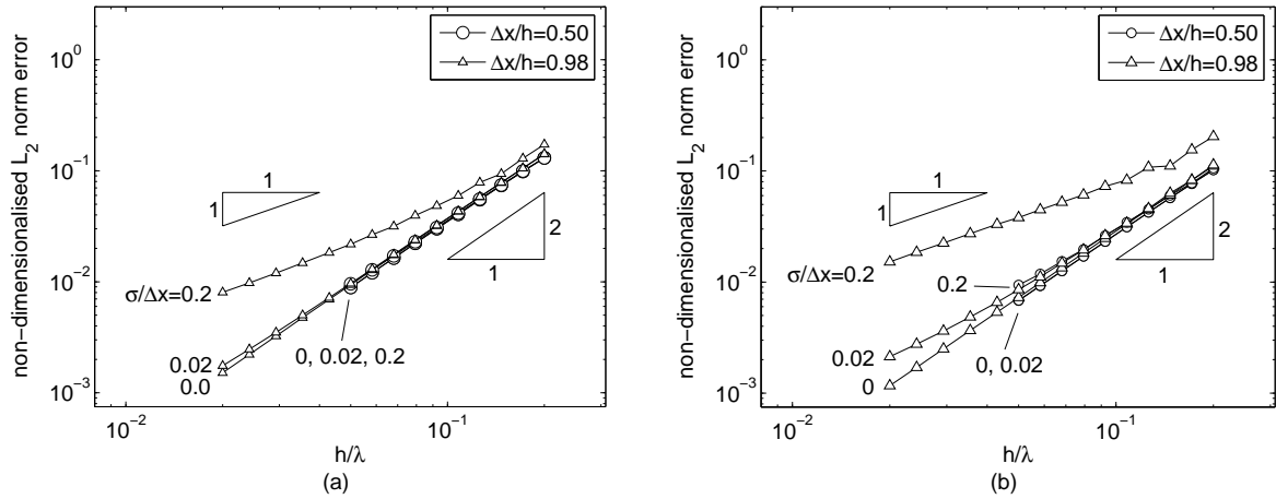
Figure 8. Observed L_2 norm error in 3D in estimates of the gradient of A(\vec{x}) = A_0 \sin(2\pi\vec{x} \cdot \vec{n}/\lambda) , for various values of mean particle spacing \Delta x/h and spacing perturbation \sigma/\Delta x , with (a) first-order consistent gradient-corrected SPH and (b) first-order consistent RKPM.
