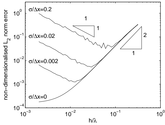
Figure 4. Observed L_2 norm error in SPH estimates of the first derivative of A(x) = A_0 \sin(2\pi x/\lambda) as a function of smoothing length, for various particle spacing perturbations, computed with \Delta x/h = 0.364 .
