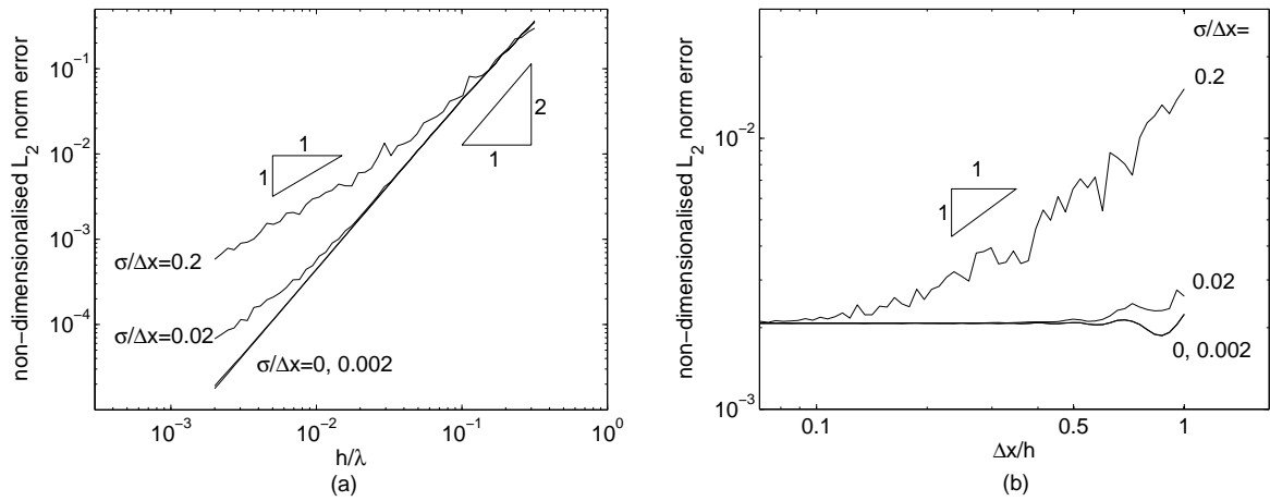
Figure 6. Empirically observed error in first-order consistent SPH gradient estimates of a sinusoidal data function for various particle spacing perturbations (a) as a function of smoothing length h with \Delta x/h = 0.7 , and (b) as a function of particle spacing ratio \Delta x/h with h/\lambda = 0.022 .
