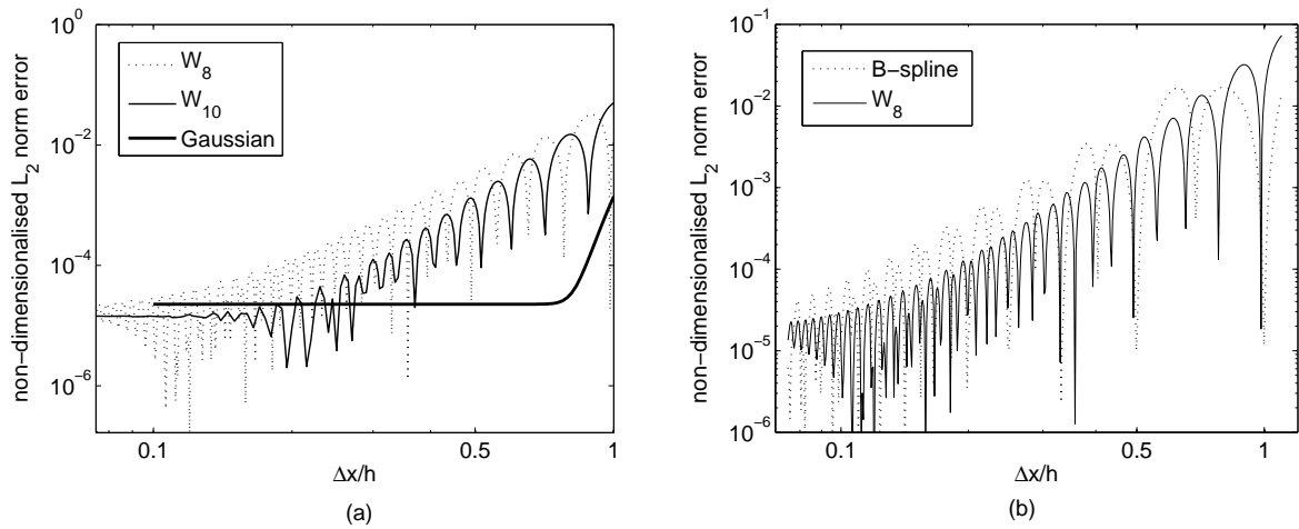
Figure 3. Observed rms error in SPH estimates of the first derivative of A(x) = A_0 \sin(2\pi x/\lambda) , for (a) 8 th -order polynomial, 10 th -order polynomial and Gaussian kernels, and (b) the B-spline and 8 th -order polynomial kernels. h/\lambda = 0.0018 in all cases.
