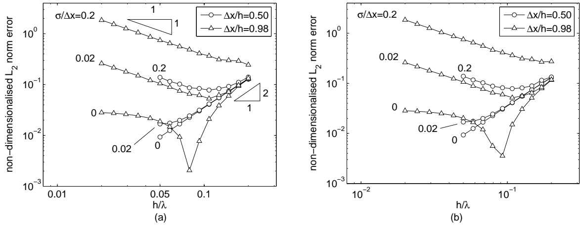
Figure 7. Empirically observed error in 3D SPH gradient estimates of a sinusoidal data function for various values of mean particle spacing \Delta x/h and spacing perturbation \sigma/\Delta x . In (a), the data gradient is aligned with the baseline unperturbed particle distribution, and in (b) it is oblique.
