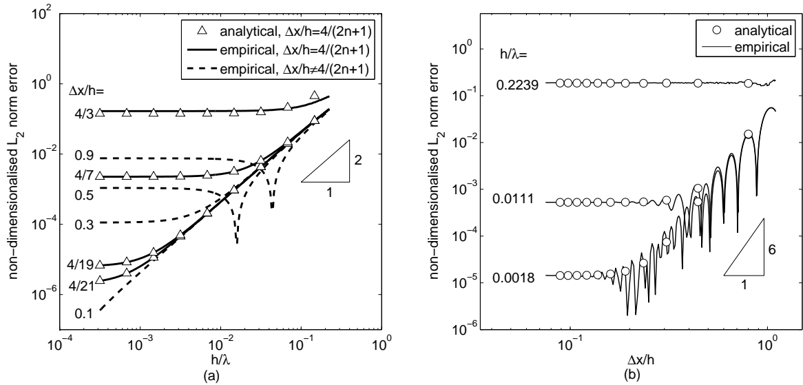
Figure 2. Analytically and empirically calculated L_2 norm of error in SPH estimates of the first derivative of A(x) = A_0 \sin(2\pi x/\lambda) (a) as a function of smoothing length for various values of particle spacing, and (b) as a function of particle spacing for various smoothing lengths.
