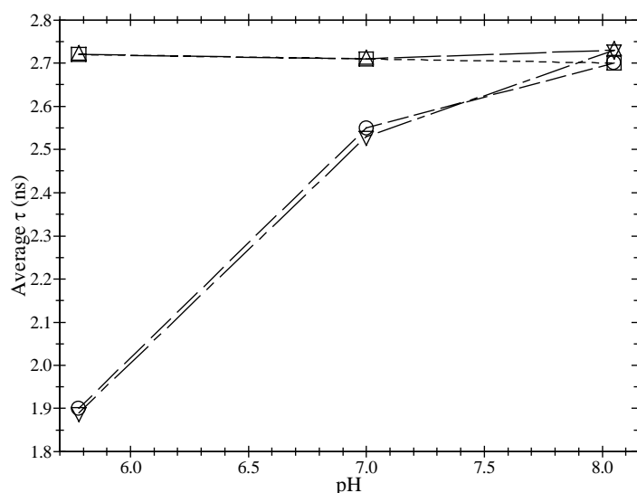
Figure 5: Average lifetime versus pH for resorufin doped TP1 at 600 nm (o) and 650 nm ( \nabla ), and TP2 at 660 nm ( \Delta ) and 650 nm ( \square ). Lifetimes were recorded in 0.1M phosphate buffer with 460 nm excitation.
